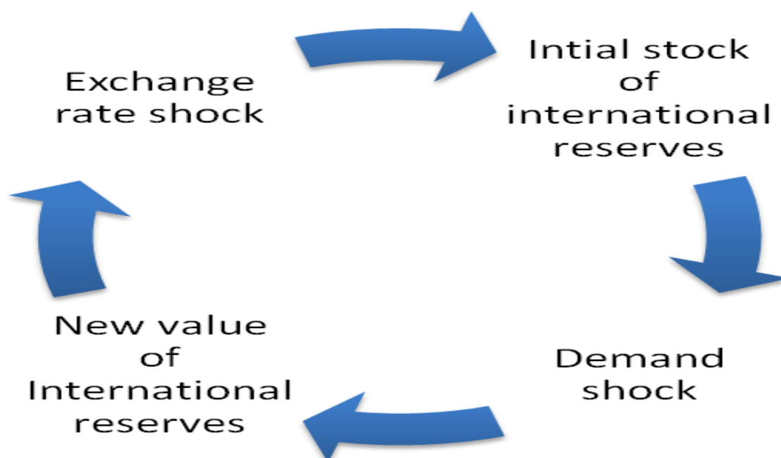
Figure 2: Representative Model of Monte Carlo Experiment
