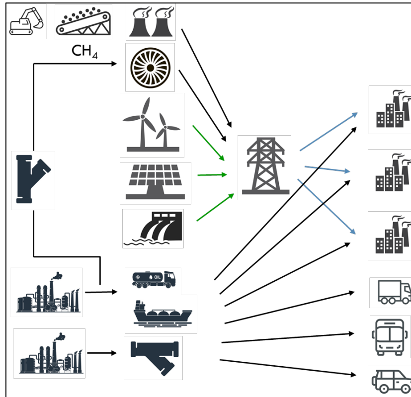
Growing Use of Variable Renewable Energy
